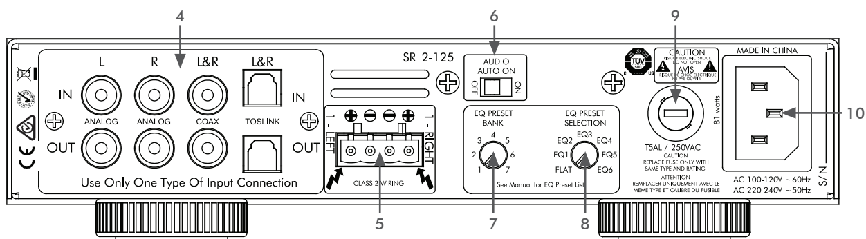
FIGURE 3: SR 2-125 TWO-CHANNEL AMPLIFIER REAR PANEL
