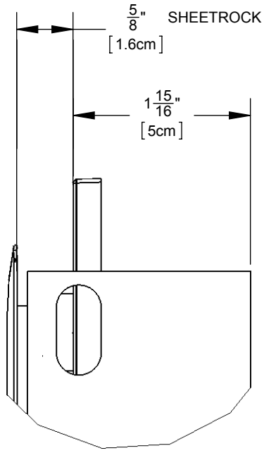
DETAIL K SCALE 2 : 3
