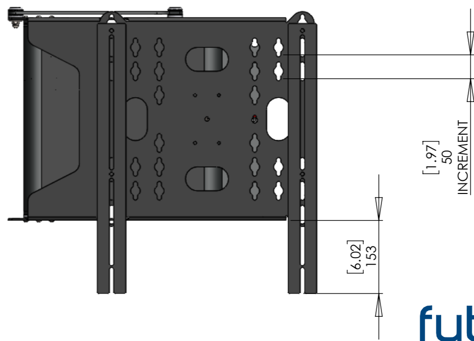
PSE90 BRACKET MINIMUM OFFSET (AT 50MM [1.97] INCREMENT)
